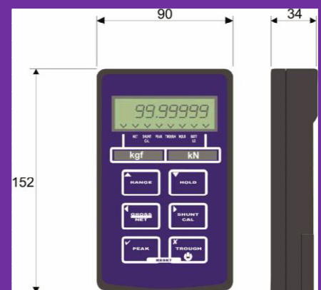
Mechanical Dimensions All dimensions in millimeters
